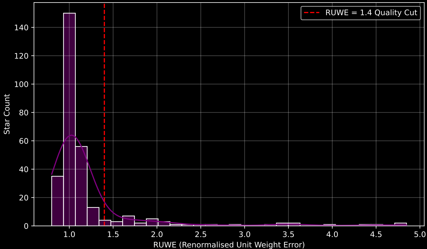
GAPOGEE DR17 Field [sgr_tidal8] RUWE Distribution (n= 293)
