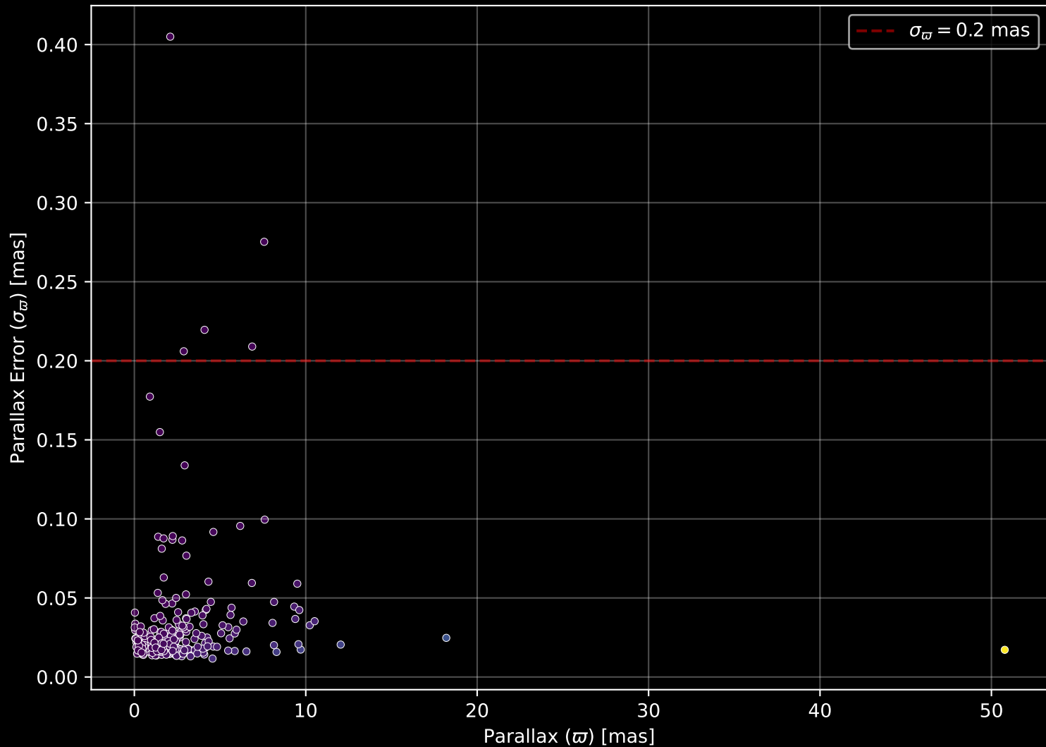
APOGEE DR17 Field: [sgr_tidal8] Parallax Quality (n= 301)
