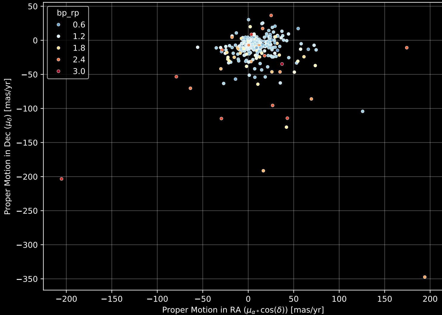
APOGEE DR17 Field: [sgr_tidal8] Proper Motion Diagram (n= 301)
