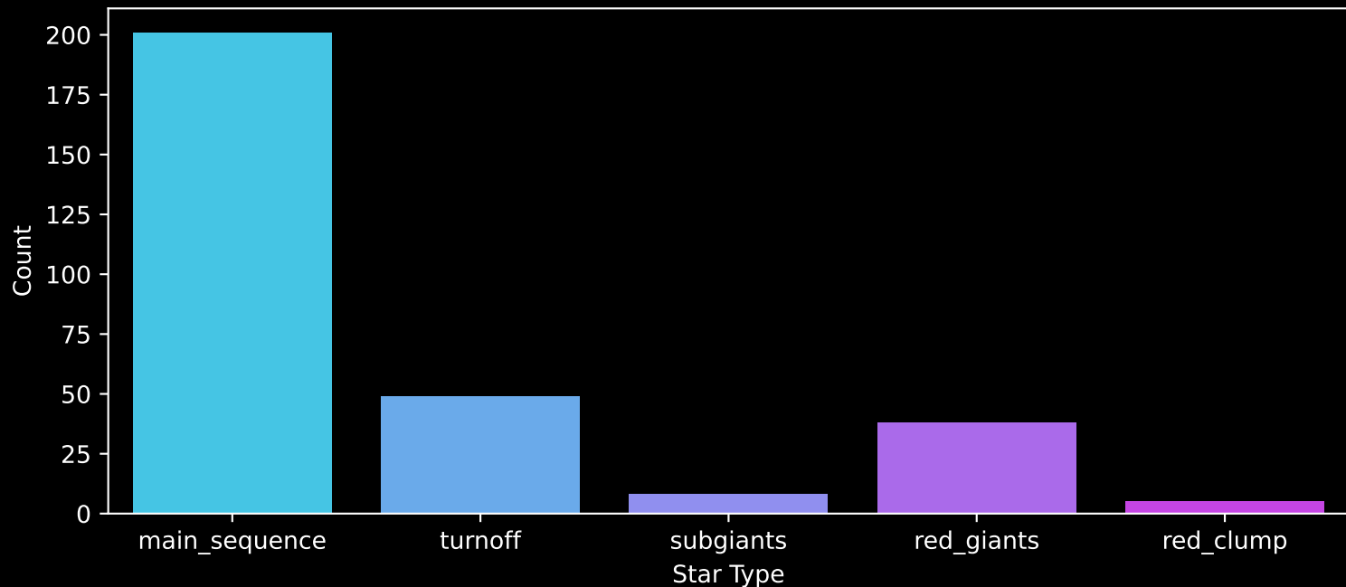
APOGEE DR17 Field: [sgr_tidal8] Count plot of Star Type
