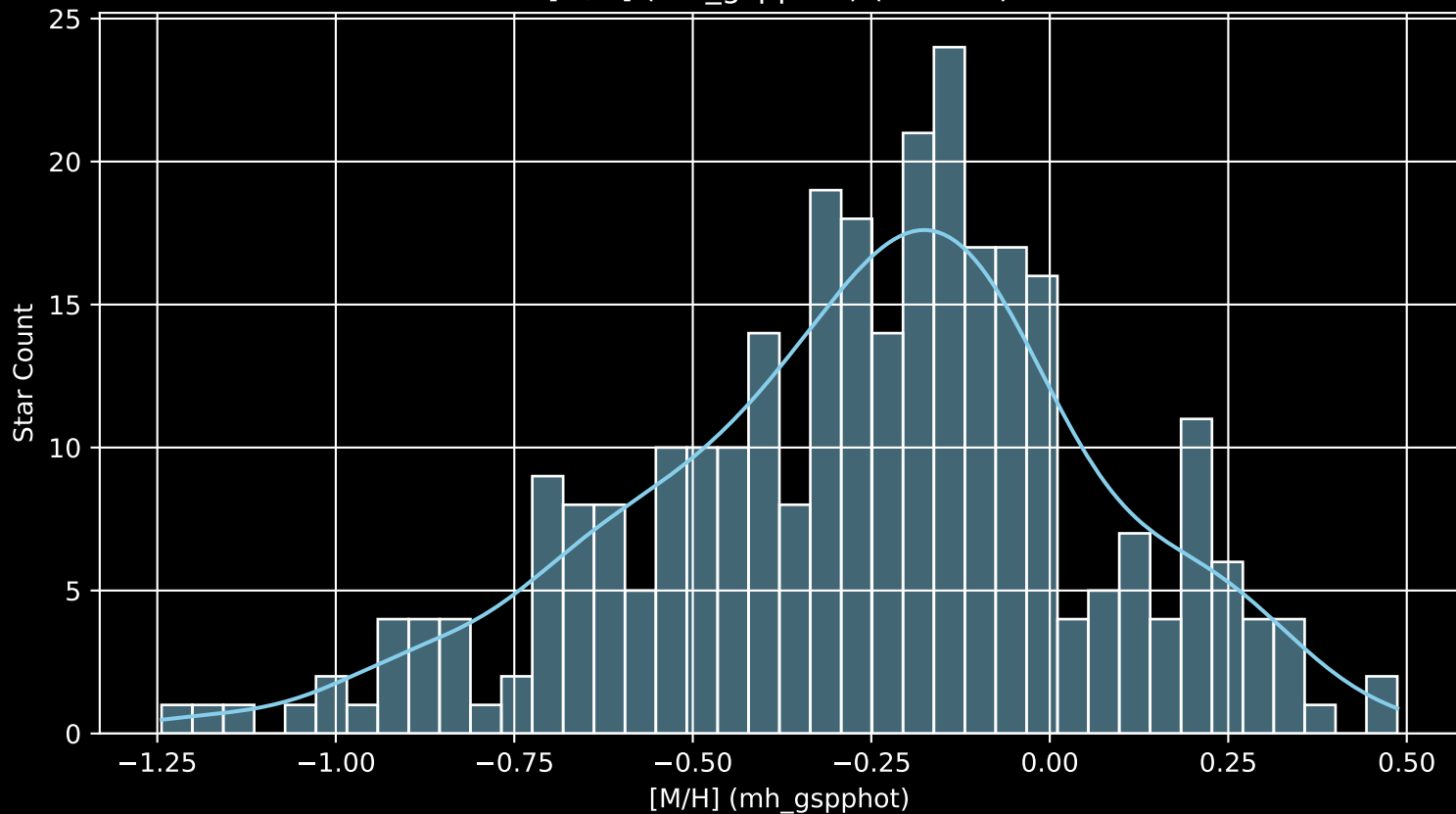
APOGEE DR17 Field: [sgr_tidal8 [M/H] (mh_gspphot) (n= 298)
